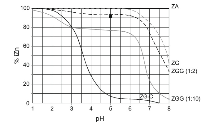
Fig. 1. Percentage of zinc present as iZn by pH. At physiologic pH 7.4, zinc acetate (ZA) yields 100% iZn, zinc gluconate (ZG) yields 72% iZn, zinc gluconate with a 1:2 M ratio of zinc gluconate to glycine [ZGG (1:2)] yields 57% iZn, zinc gluconate with a 1:10 M ratio of zinc gluconate to glycine [ZGG (1:10)] yields 11% iZn, and zinc gluconate with a 1:1.3 M ratio of zinc gluconate to citrate or zinc citrate (ZG–C) yields zero iZn.
