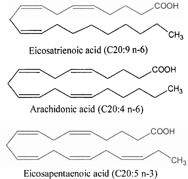
20-Carbon fatty acid homologues.
